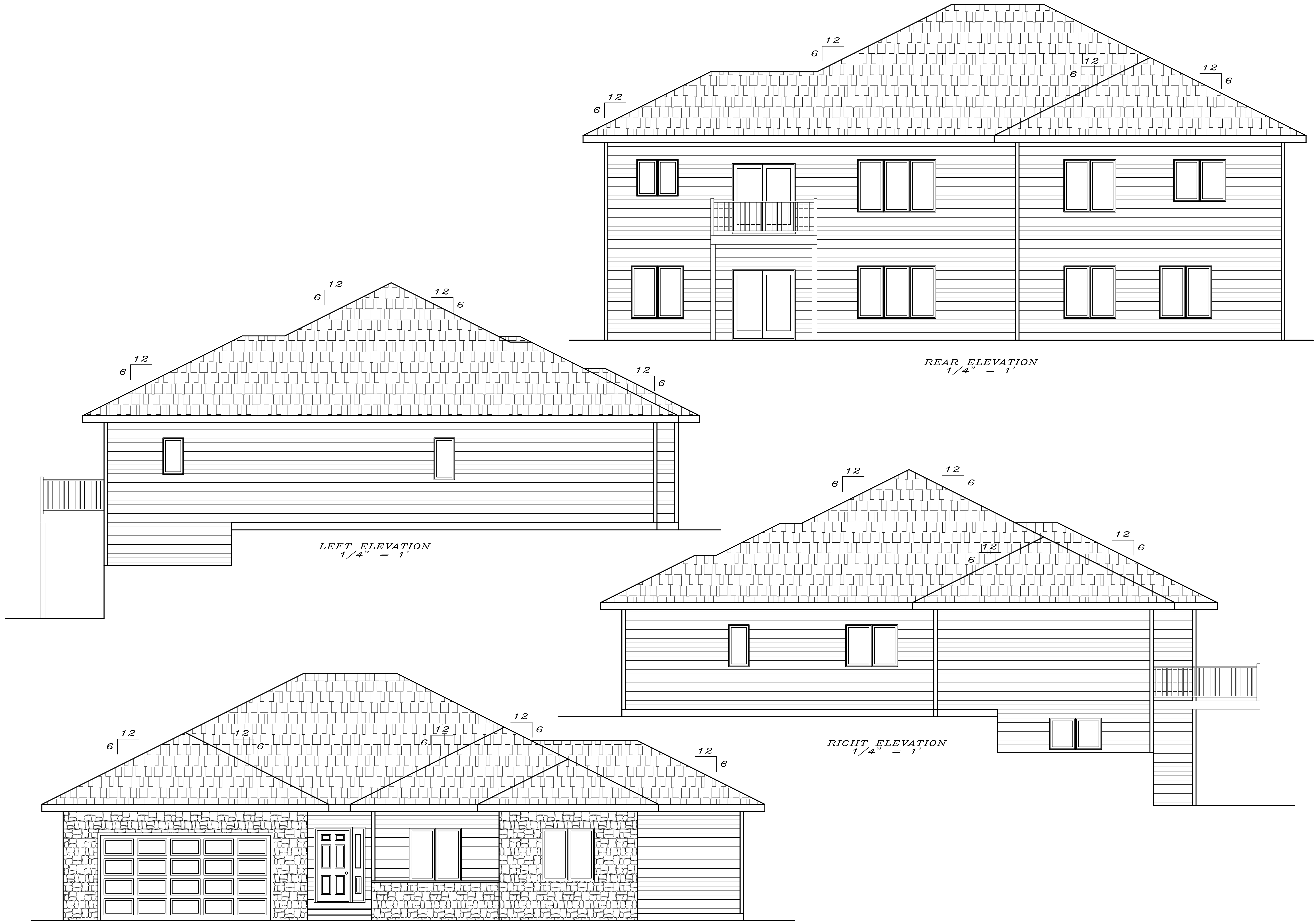
FRONT ELEVATION 1/4" = 1'
